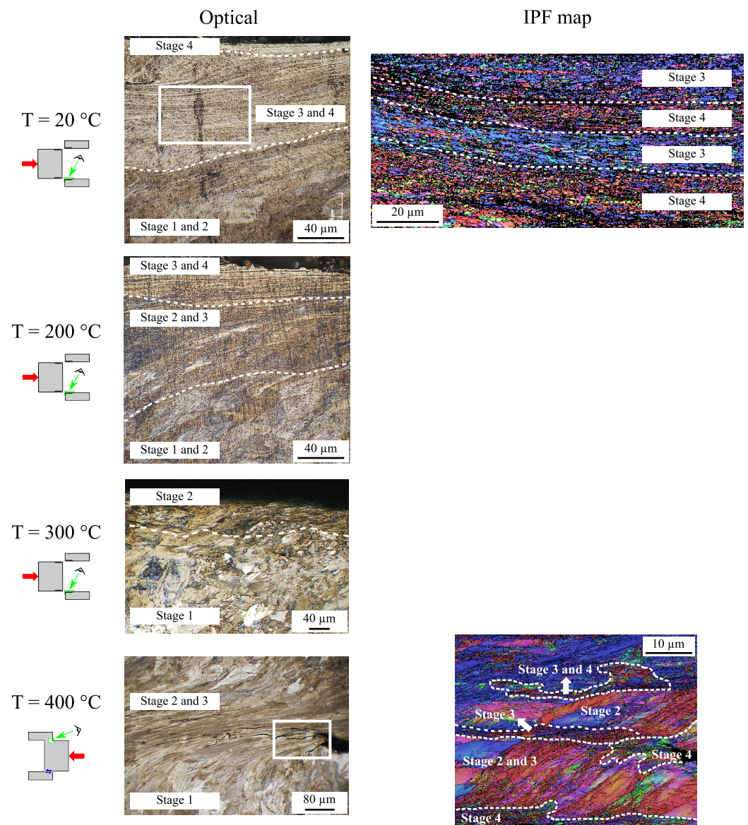
Figure 9. Effect of temperature on the microstructural gradient in the sheared zone of the specimen at the end of the monotonic tests. The specimen failed at the tests performed at T = 20\text{ °C} , 200\text{ °C} , and 300\text{ °C} but did not fail at 400\text{ °C} . IPF maps were constructed for the tests performed at room temperature (step size = 0.08\text{ }\mu\text{m} ) and 400\text{ °C} (step size = 0.1\text{ }\mu\text{m} ).
