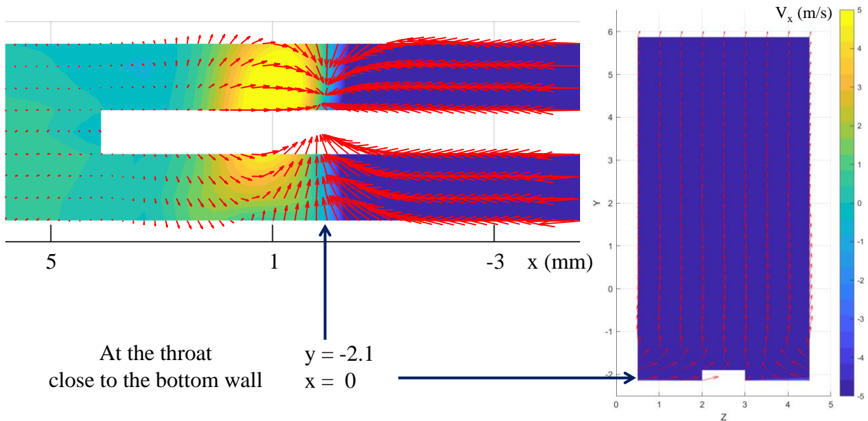
Figure 16. Zoom at the flow field close to the bottom wall, immediately downstream from the throat: velocity vectors and V_x (color field) in the x-z plane located at y = -2.1 mm (left) and in the y-z plane located at x = 0 (right) for test case #4
