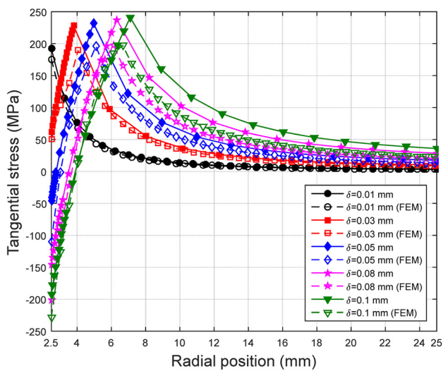
Fig. 7 Hoop stresses—during loading
