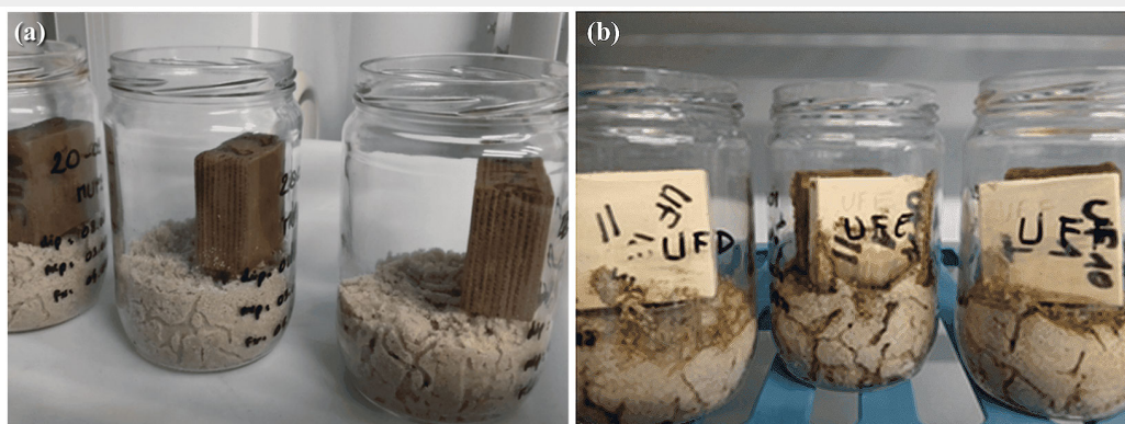
Fig. 2 - Termite resistance tests of untreated and heat-treated poplar plywood samples: (a) non-choice test devices and (b) choice test devices.
