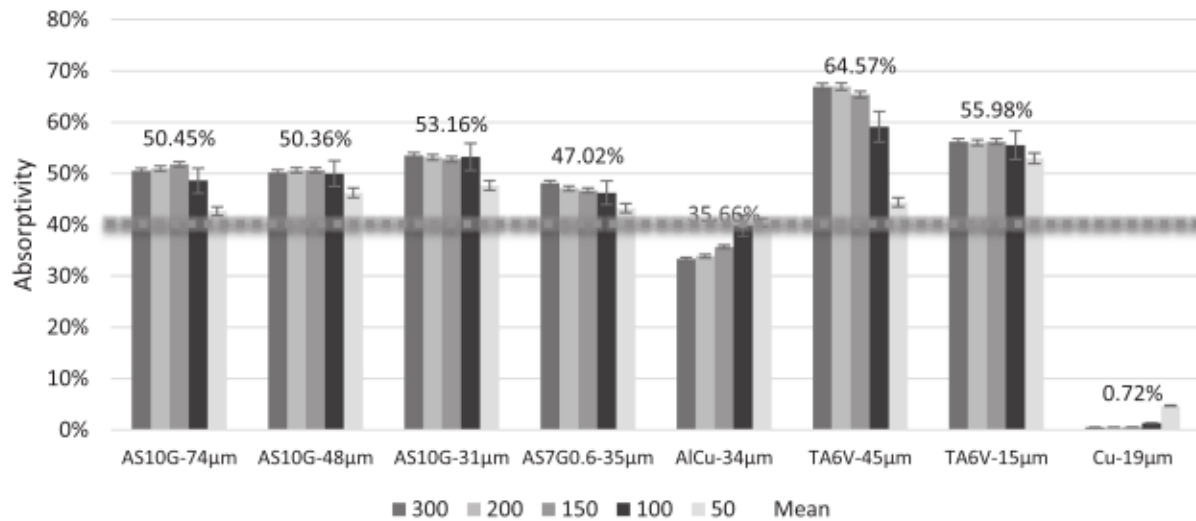
Fig. 8. Average absorptance measurements for several powders and material for \phi 2 mm - powder bed layer thickness from 50 to 300 \mu m - highlighted values: mean - line: absorptivity of the substrate.
