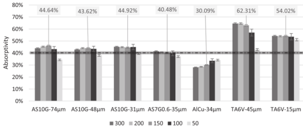
Fig. 9. Average absorptance measurements for several powders and material for \phi 0.2 mm - powder bed layer thickness from 50 to 300 \mu m - highlighted values: mean - line: absorptivity of the substrate.
