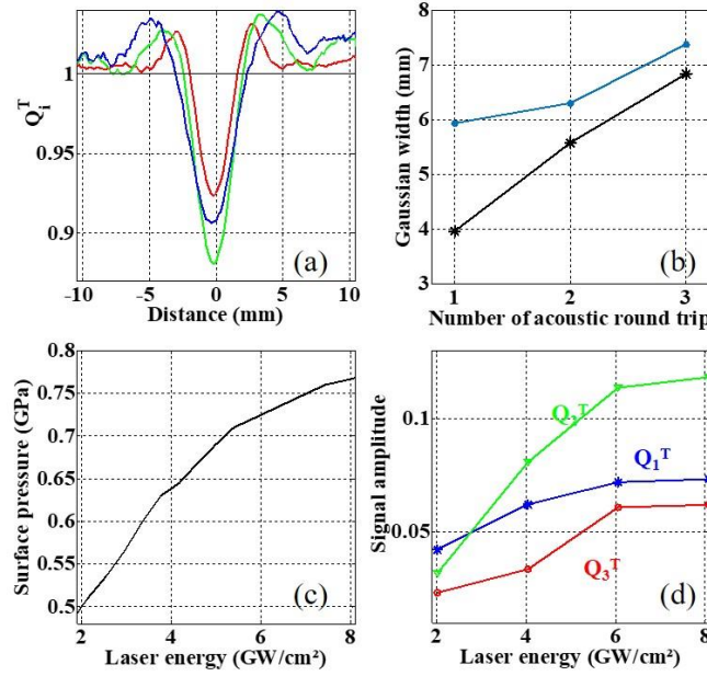
Figure 4 : (a) Average detection of Q_i^T ( i=1 (red), 2 (green), 3 (blue)). (b) FWHM of Q_i^T for a laser focus of 3 mm (black stars) and 5 mm (blue points) diameter. (c) Laser pressure loadings as function of the laser intensity from ESTHER simulations. (d) Intensity of the detected signal Q_i^T , i = 1 to 3, as function of the laser intensity.
