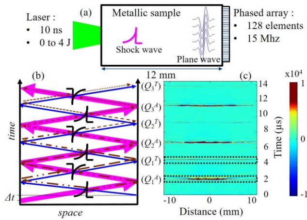
Figure 2: (a) Principles of experiments. (b) Space time representation : shock (plane wave) propagation is represented by the purple (blue) arrows and diffracted signals by dashed arrows. (c) Time-space PA detection of the pressure field. The dotted line rectangles illustrate the temporal integration on the acoustic echoes for the investigation procedure.
