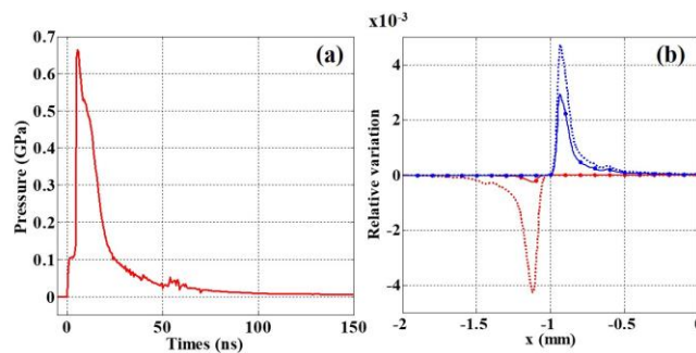
Figure 1 : (a) Surface pressure induced by a ns laser pulse in aluminum. (b) Simulations of the density (dashed lines) and velocity (symbols) relative variations in a 2 mm thick plate, 300 ns (blue) and 450 ns (red) after generation.
