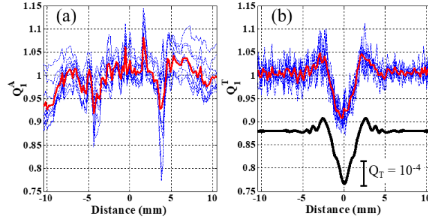
Figure 3 : Detection of ratio Q_1^A (a) and Q_1^T (b) from single shot detection (dot blue lines) and averaging of 10 detections (red continuous line). On (b), the signal presented in black (with its own amplitude scale) is obtained from linear simulations of a static inclusion.
