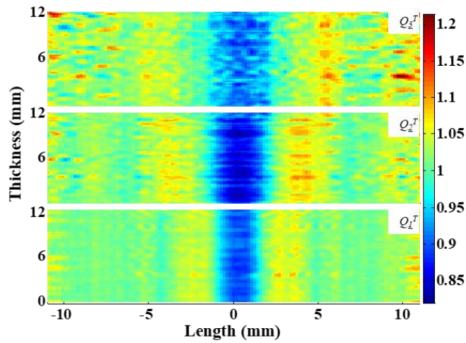
Figure 5 : Elastography of the shock wave propagation during three round trips in the material.
