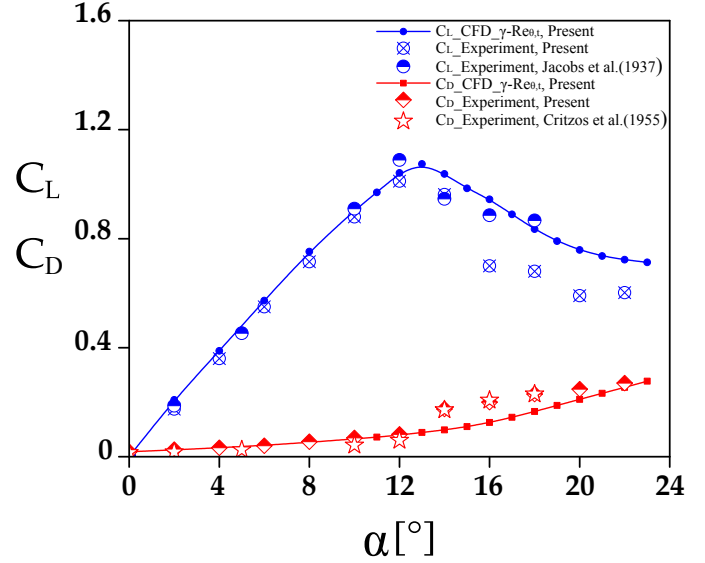
Figure 11: Comparison between the current CFD and experimental results with previous experimental data.
