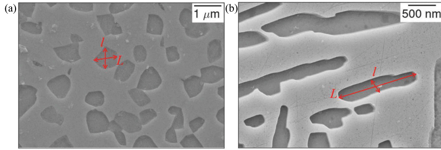
Fig. 1. Method to measure the size of \alpha particles.
