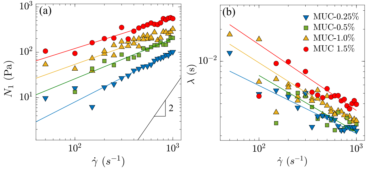
Fig. 2. (a) First normal-stress difference as a function of shear rate. Data are fitted with a power law model. Black solid line of slope \alpha = 2 represents the Oldroyd-B model ( N_1 = 2\eta_p\lambda\dot{\gamma}^2 ), considering an identical relaxation time at polymer contribution to the zero shear viscosity \eta_p . (b) Relaxation time as a function of shear rate for different concentration of synthetic mucus using the White–Metzner model. Colored continuous lines are fitted to the experimental data by a power law model. The corresponding model constants can be found in Table 1.
