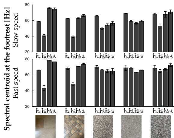
Figure 6. Spectral centroid computed at the footrest of the tested MWC over all the propelling conditions. 1: Empty MWC pushed by an assistant; 2: MWC loaded with a dummy and pushed by an assistant; 3: MWC loaded with a non-pathological participant and pushed by an assistant; 4: MWC loaded with a self-propulsing non-pathological participant.
