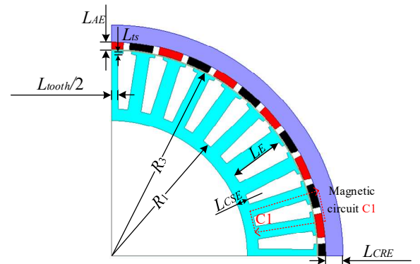
Fig. 3. Motor radial dimension drawing
