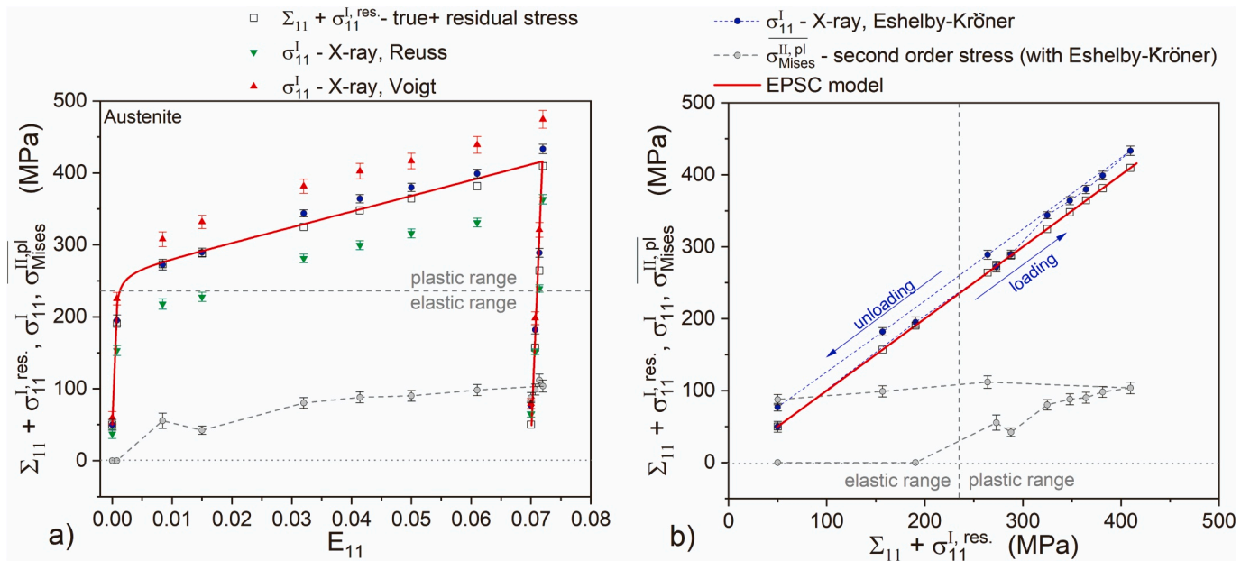
Fig. 11. Evolution of the experimental first-order stresses expressed in two ways: \sigma_{11}^I and \sigma_{11}^{I, res} + \Sigma_{11} compared with \sigma_{11}^I predicted by the EPSC model, using parameters given in Table 3, for an austenitic sample subjected to tensile deformation. The evolution of determined second-order stresses mean von Mises stress ( \sigma_{Mises}^{II, pl} ) is also presented. The plots vs. sample strain E_{11} (a) and first-order stress \Sigma_{11} + \sigma_{11}^{I, res} (b) are shown.
