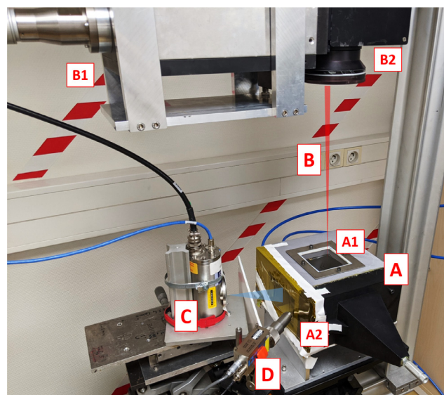
Fig. 2. Photography of the setup with the interaction chamber (A); the laser (B1) and the scanning head (B2); the X-ray tube (C) and the spectral detector (D).
