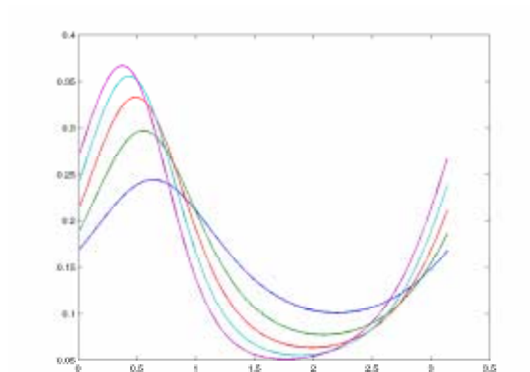
Figure 2. Reduced approximation modes related to the evolution of the orientation distribution function along a flow streamline.
