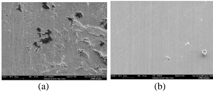
Fig 7: SEM photos of the machined surfaces in (a) CM and (b) LAM.
