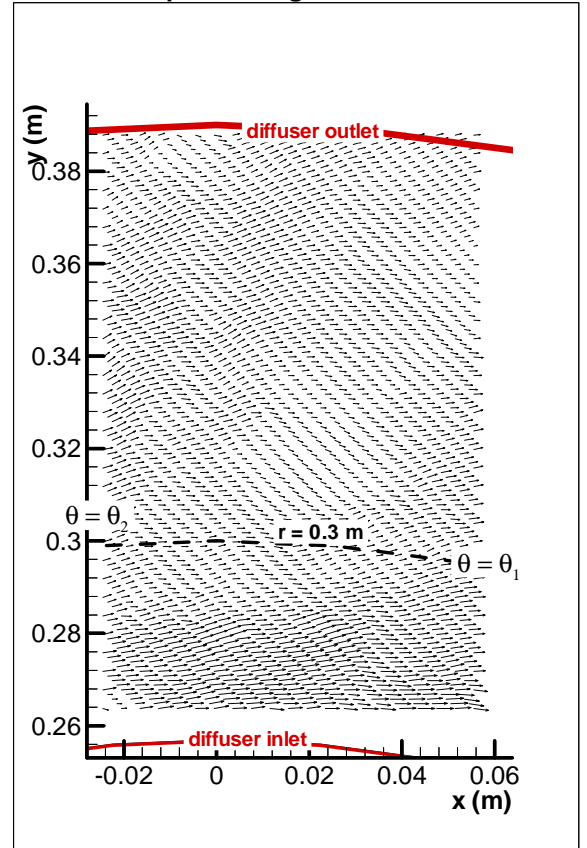
Fig 5 : Example of velocity map and of a line ( r = 0.3 m ) on which the average value of the velocity component are performed.
