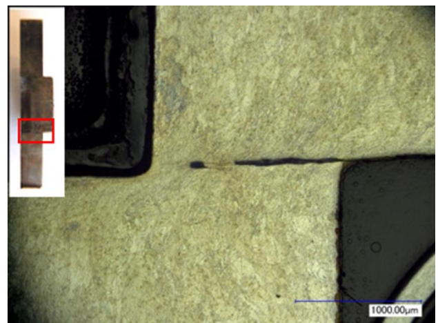
Fig. 8: microstructural observation after a shear test performed with a strain rate of 5 \cdot 10^4 \text{ s}^{-1} at a temperature of 400°C
