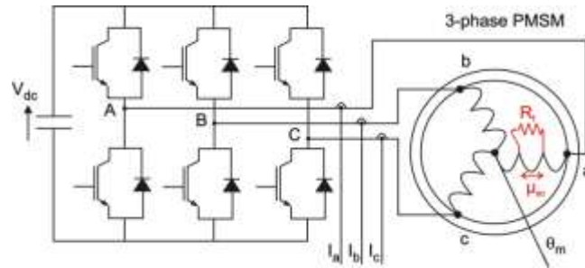
Fig. 1 PMSM drive with an inter-turn fault
