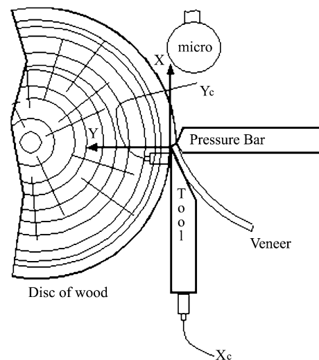
Fig. 3 Experimental setup
