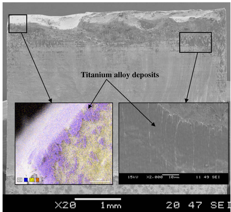
Fig. 4. SEM images of a 0° rake angle tool under a cutting speed of 60 m/min and a feed of 0.3 mm.
