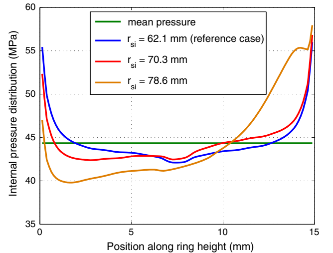
Fig. 7. Pressure distribution for three different positions of the support.
