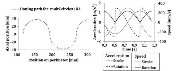
Fig. 5. Sinusoidal honing path with speed and acceleration.
