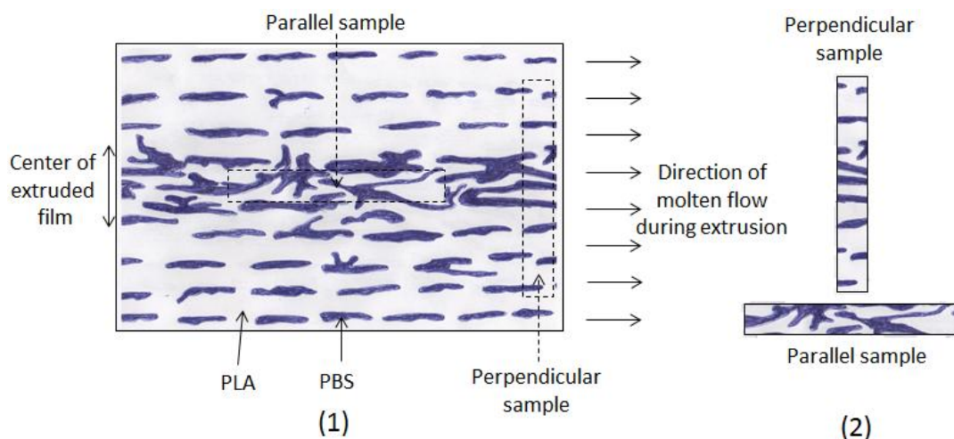
Figure 4. Molten film of PLA/PBS blend during extrusion (1); perpendicular and parallel samples (2).
