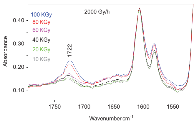
Fig. 4. FTIR spectra of epoxy/POPA during radiochemical ageing normalized at 1606\text{ cm}^{-1} for 50, 200 and 2000 Gy/h doses rates.
