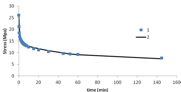
Figure 5. Stress–relaxation test on PU specimen at 30°C: Experimental results (1), Modified Maxwell–Weichert model (2). [Color figure can be viewed in the online issue, which is available at wileyonlinelibrary.com .]
