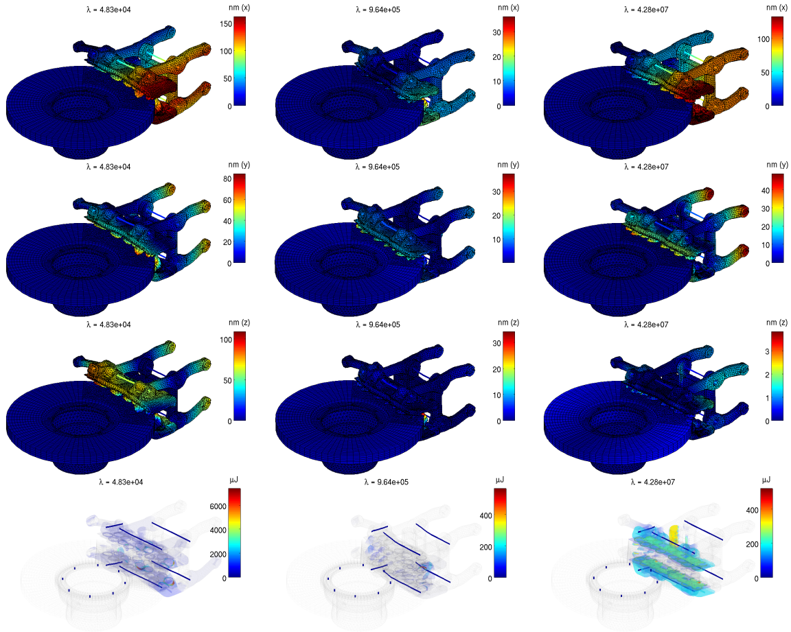
Figure 14: Absolute displacement differences in nanometers between Signorini and functional static results, from top to bottom along the x , y and z axis, from left to right in increasing \lambda . Strain energy densities of differential displacements are presented for elements with highest levels only
