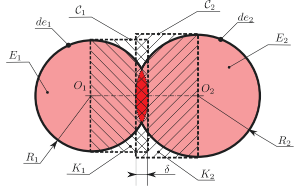
FIGURE 5: The contact model between two discrete element silica
