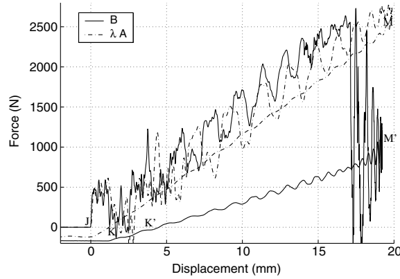
Fig. 13. Comparison between measured force and similitude law result (vs time) at V_{\text{init}} = 2.2 \text{ m s}^{-1} .
