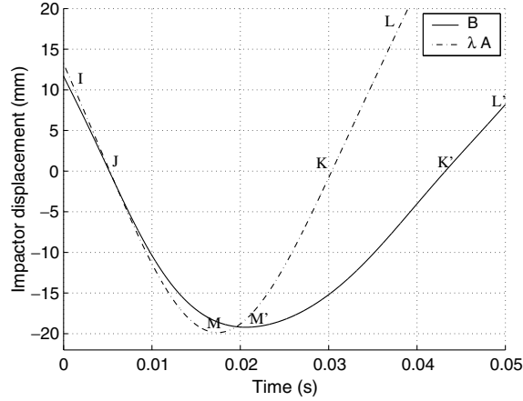
Fig. 12. Comparison between measured impactor displacement and similitude law result (vs time) at V_{\text{init}} = 2.2 \text{ m s}^{-1} .
