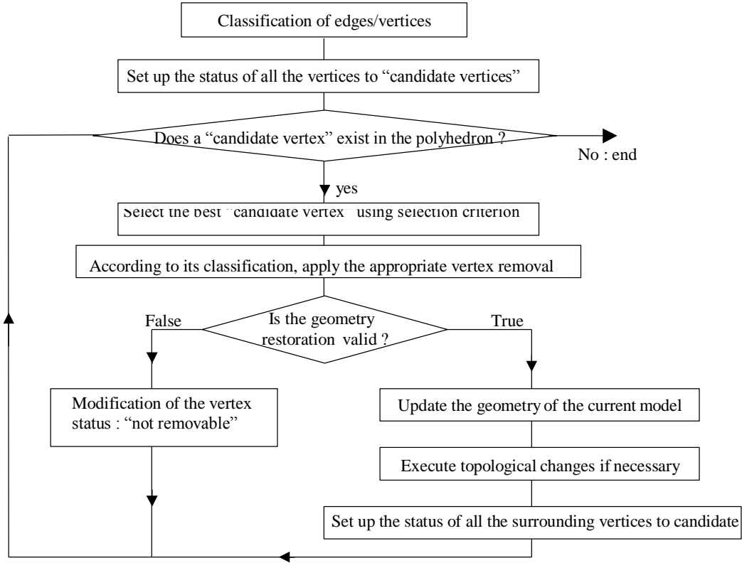
Figure 1 : The main steps of the simplification loop algorithm.
