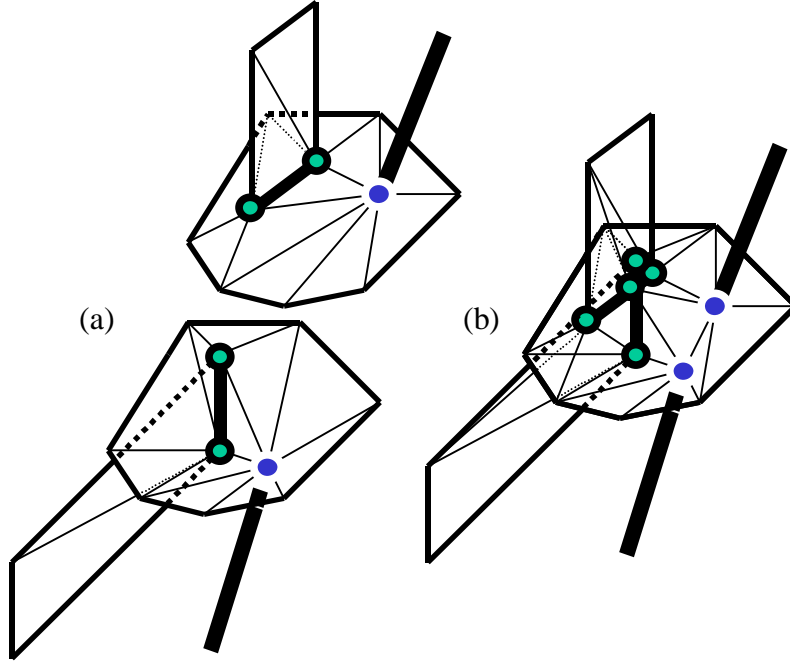
Figure 15 : Constrained re-meshing process applied when both half-surfaces are connected to other geometric elements : (a) the two half-surfaces, (b) result of the constrained re-meshing process.
