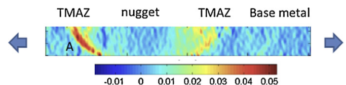
Fig. 4. Speckle deformation map of the sample through-thickness section ( F = 2.8 kN), the A symbol indicates the advancing side location.
