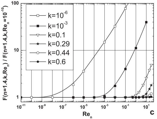
Fig. 4. Influence of the confinement on the critical Reynolds number marking the rise of the inertia: (a) for n = 0.6 , (b) for n = 0.9 , (c) for n = 1.4 .
