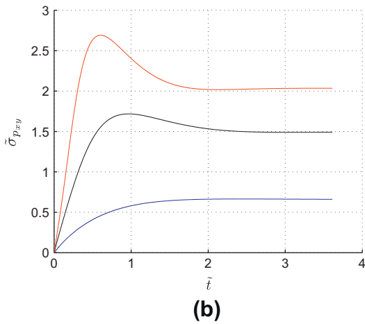
Fig. 3. Start-up plane Couette flow: shaded surface of the equilibrium PDF for Wi_m = 5 on a 1681 DoF lattice (a) and dimensionless shear stress evolution \tilde{\sigma}_{p_{xy}} for different Wi_m on a D2Q9 lattice with 3721 DoF and \tau = 0.55 (b).
