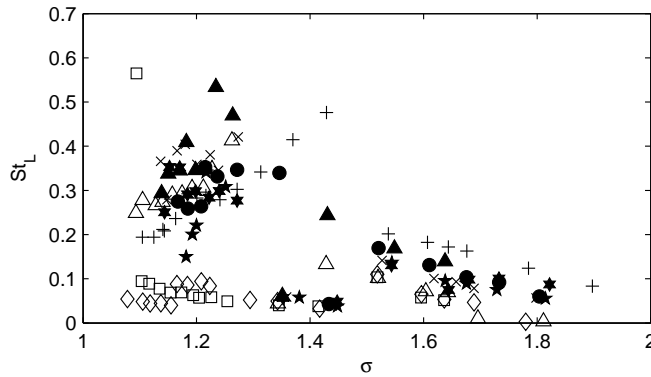
Fig. 13. Strouhal number St_L = \frac{Lf_L}{v_{throat}} according to the cavitation number \sigma : \times : plate 0, \star : plate 1, \triangle : plate 2, \ast : plate 3, + : plate 4, \blackstar : plate 5, + : plate 6, \diamond : plate 7, \square : plate 8.
