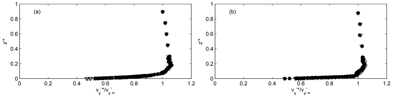
Fig. 16. Longitudinal non-dimensional velocity profile v_y^*/v_{y\infty}^* of the non-cavitating flow, at y^* = 0.5 , for (a) the grooved sheet 6 and (b) the grooved sheet 2. \bullet : x^* = 0 , \triangle : x^* = \frac{\lambda}{2}
