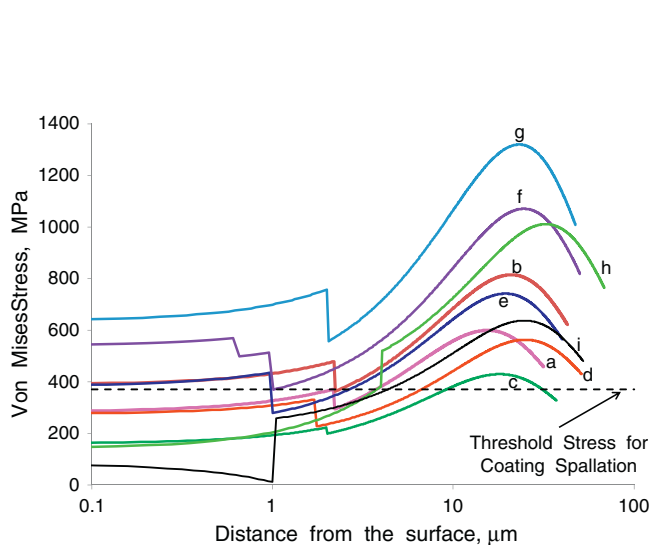
Fig. 7. Variation of the von Mises stress with the distance from the surface for the systems under study and for other DLC coated systems reported in the literature and described in Table 2.
