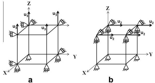
Fig. 1. Single element and boundary conditions for tests: (a) uniaxial tension and (b) simple shear.
