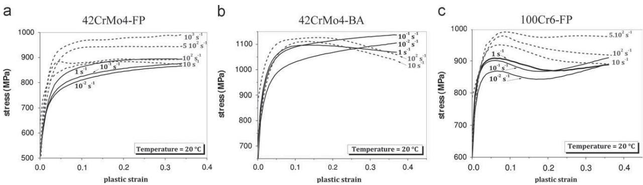
Fig. 10. Evolution of the compressive stress as a function of the plastic strain at 20\text{ °C} for different strain rates. Comparison between the three steels studied.
