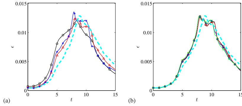
Fig. 7 Influence of the SGS model for the Taylor-Green vortex. (a) Smagorinsky-type models. Kinetic energy dissipation \epsilon for: (—○) SM with C_S=0.18 ; (—△) SM with C_S=0.1 ; (—*) DSM. (b) Multi-scale Smagorinsky models. Kinetic energy dissipation \epsilon for: (—○) MSM-ss; (—△) MSM-ls; (—*) MDSM-ss; (—□) MDSM-ls. (—□) 256^3 (see Fig.3).
