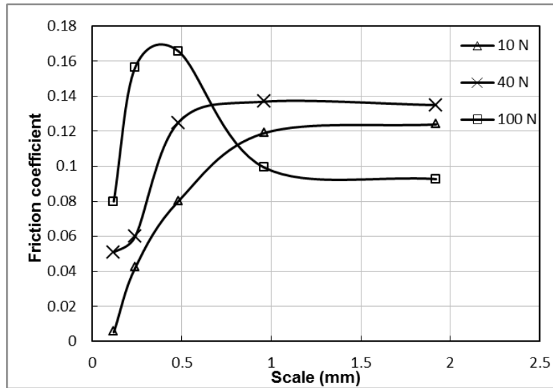
Fig. 6. Fiction coefficient as a function of scale for u_1 = 0.5 \text{ m.s}^{-1} and Srr = 2.0 .
