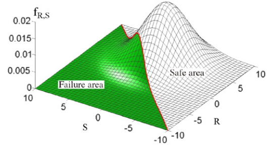
Fig. 4. Density of joint probability.
