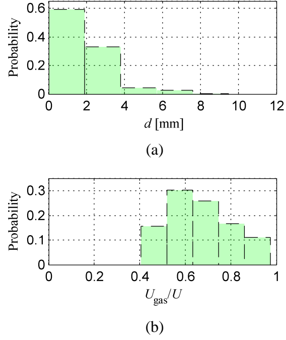
Fig. 15. (a) Bubble size histogram and (b) bubble velocity histogram at x = 5H and y = 0.615H for q = 4.60 \times 10^{-3} and three different runs of 30 seconds. The mean bubble size based on the bubble size histogram obtained by the inverse method is 1.9 mm.
