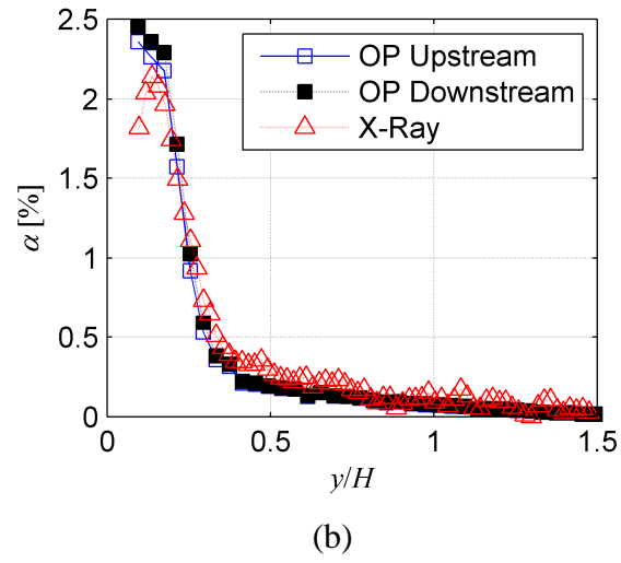
Fig. 21. (a) A comparison of the measured void fraction by all three methods for q = 1.64 \times 10^{-3} at x = 21H . (b) Comparison of the void fraction based on the optical probe and x-ray data for q = 4.60 \times 10^{-3} at x = 21H .
