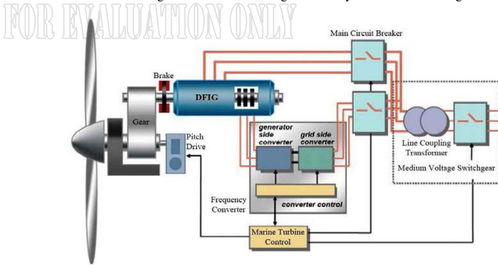
Fig. 6: Schematic diagram of a DFIG-based generation system
