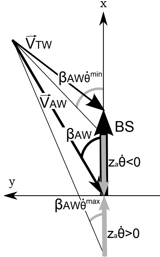
Figure 6: Dynamic effect of pitching on the wind triangle (top view). \vec{V} is the wind velocity, BS is the boat speed, z is the height of the aerodynamic centre of effort, \dot{\theta} is the pitching velocity, \beta is the apparent wind angle, subscripts TW and AW stand for True and Apparent wind
