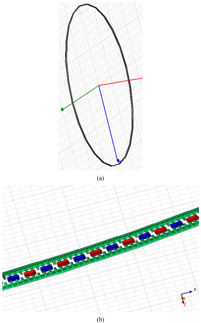
Fig. 8. (a) Representation of the sized DSAFPM machine active part volumes and (b) zoom on an arc of the machine.
