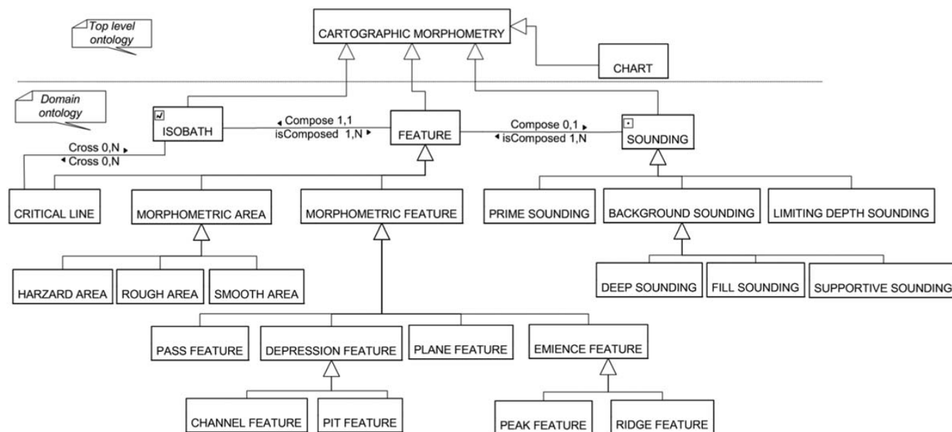
Figure 9. Conceptual model of the seafloor representation
