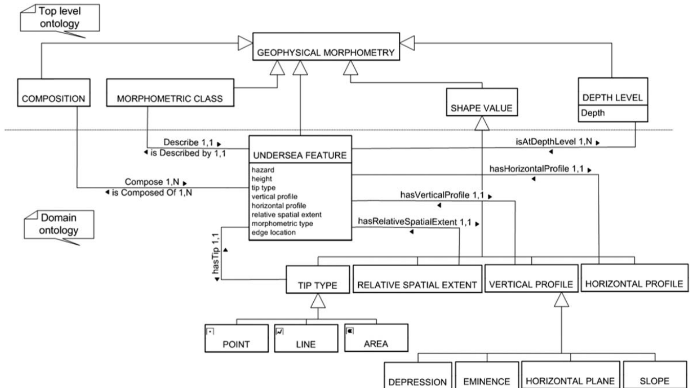
Figure 3. Conceptual model of the submarine relief 5
