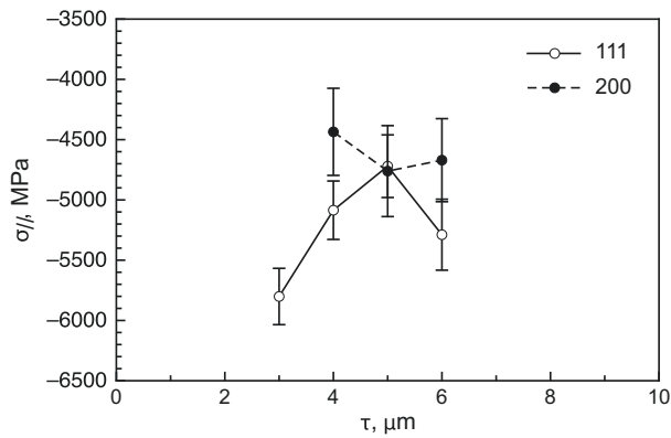
Fig. 6. Residual stress-depth profiles \sigma_{//} evaluated from 111 to 200 diffraction lines of expanded austenite from the \sin^2\psi plots at chosen information depths, \tau , reconstructed from lattice-spacing-depth profiles ( d_{\psi}^{||} ) measured from the scattering vector method applied to a nitrided 316 L stainless steel.
