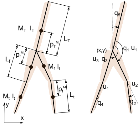
Figure 2: 5-link planar biped robot.
