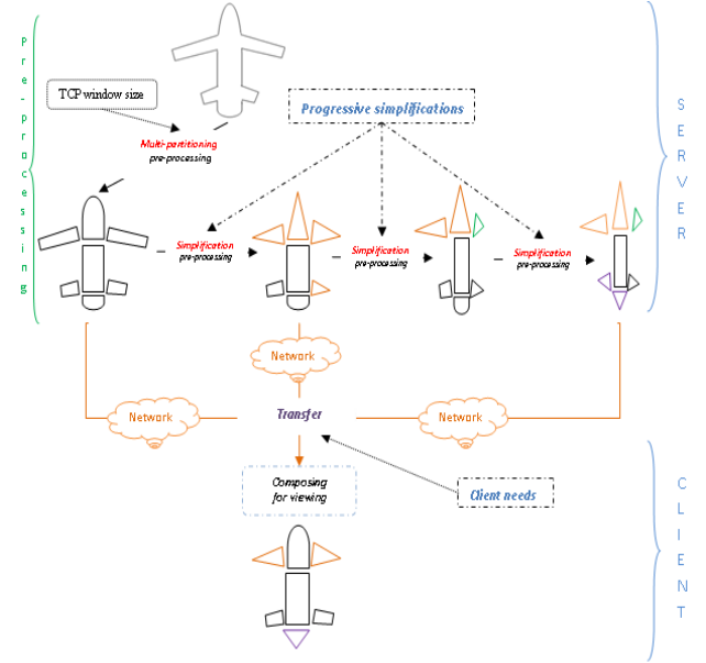
Figure 1 : architecture of proposed approach.
