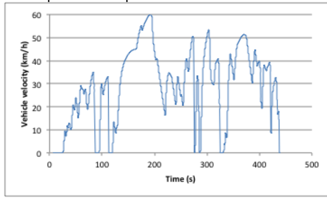
Fig. 3. Vehicle velocity
