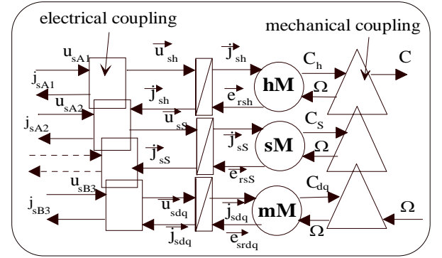
Fig 8: EMR of six-phase machine after magnetic decoupling
