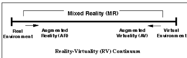
Fig. 2 Milgram's continuum [5]
